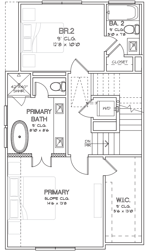
THIRD FLOOR
