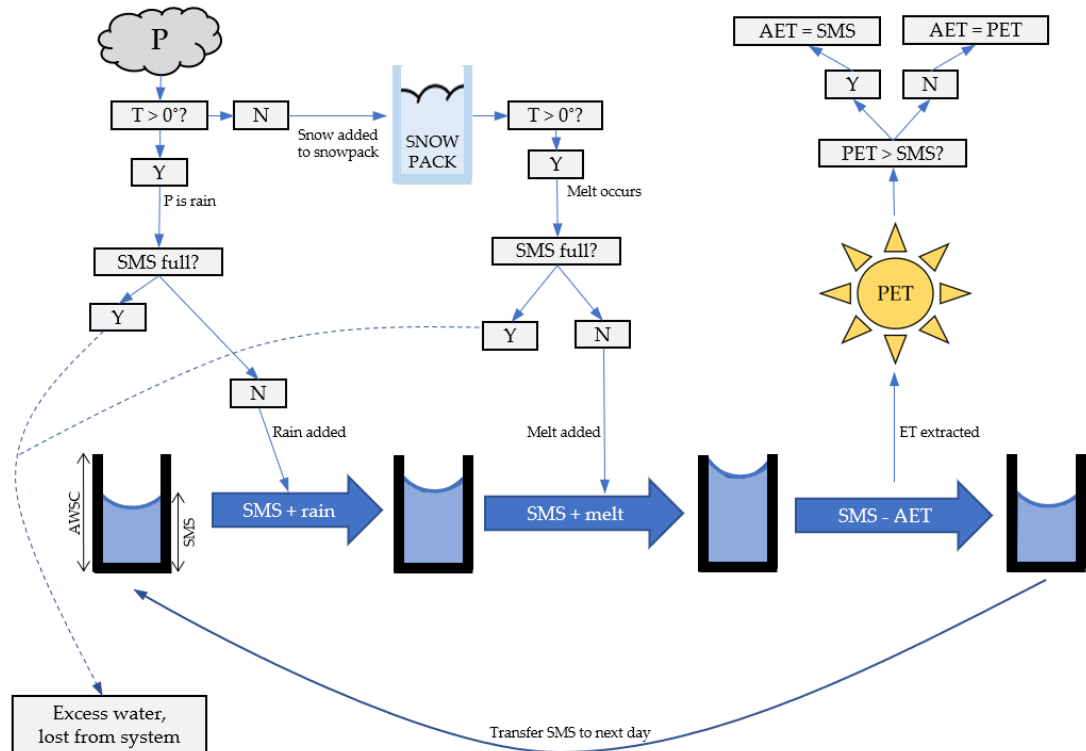
Figure 3-3. Diagram of the filling-bucket model used to estimate site water balances. The diagram depicts one daily timestep, at the end of which the soil moisture storage (SMS) is transferred to the beginning of the next day. The volume of the filling bucket is equal to the available water storage capacity (AWSC), and SMS is always equal to or less than the AWSC with excess input water lost from the system. The type of precipitation (P) and the occurrence of snowmelt are dependent on the mean daily temperature (T). Temporary storage in the field capacity-saturation pores is not shown in the diagram but occurs before excess water is lost from the system.
