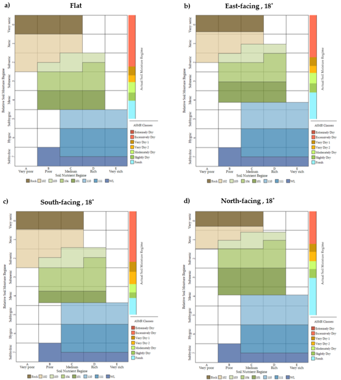
Figure 3-4. The edatopic grid for the ESSFdk1 variant (MacKillop et al., 2018) for a) flat sites (as published), b) east-facing sites on 18° slopes, c) south-facing sites on 18° slopes, and d) north-facing sites on 18° slopes.
