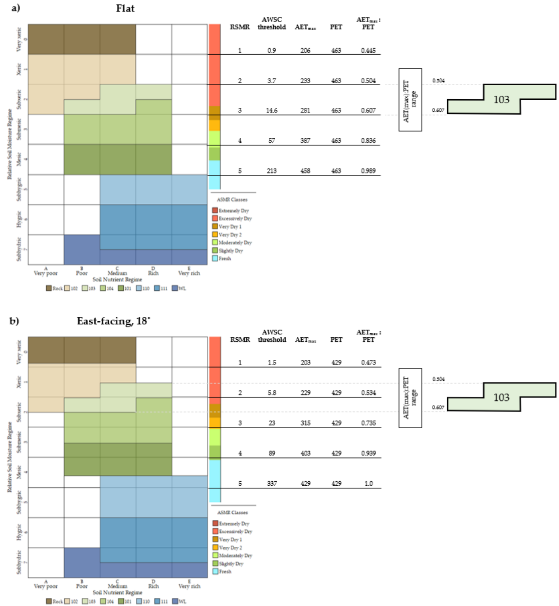
Figure 3-5. Edatopic grids for the ESSFdk1 variant (MacKillop et al., 2018) for flat and east-facing sites annotated with AWSC thresholds, AET_{max} and PET values (in mm), and AET_{max}:PET ratios at each upland RSMR class boundary. The range of AET_{max}:PET ratios for the 103 site series is given at right in order to illustrate that it maintains the same AET_{max}:PET ratio boundaries as the edatopic grid is shifted, which is also true for all other site series.
