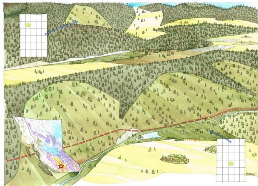
Figure 2-1. Illustration of biogeoclimatic ecosystem classification concepts. The inset map shows occurrence of broad biogeoclimatic zones across the province. The illustration depicts a landscape-scale example at a location marked by the star in the inset map, with the red dashed line indicating a boundary between biogeoclimatic subzones. The inset edatopic grids correspond to two hypothetical sites indicated by the blue arrows. The higher-elevation site sits on a steep, upper slope position, and likely would have coarser soils than the lower-elevation site. Therefore, it is represented on the edatopic grid in a drier moisture regime and poorer nutrient regime (i.e., the upper-left of the grid). The lower-elevation site is on a gentler slope in a water receiving position, and, therefore, is in a wetter and richer position on the edatopic grid (i.e., lower [wetter] and further right [richer] than the upper site).
