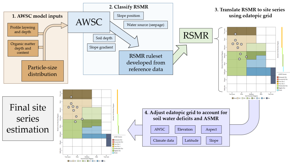
Figure 3-1. The structure of the Quantitative Ecohydrological Analysis (QEA) model used to make estimations of site characteristics. Step 1 describes the data inputs required to calculate plant-available water storage capacity (AWSC). Step 2 shows the use of AWSC and site factors to predict relative soil moisture regime (RSMR). Step 3 illustrates how estimated RSMRs are applied to regional edatopic grids to estimate site series outcomes. Step 4 shows how the published edatopic grid is adjusted to account for water-balance effects related to topography (slope, aspect, latitude), site location within a subzone, and climate change scenarios.
