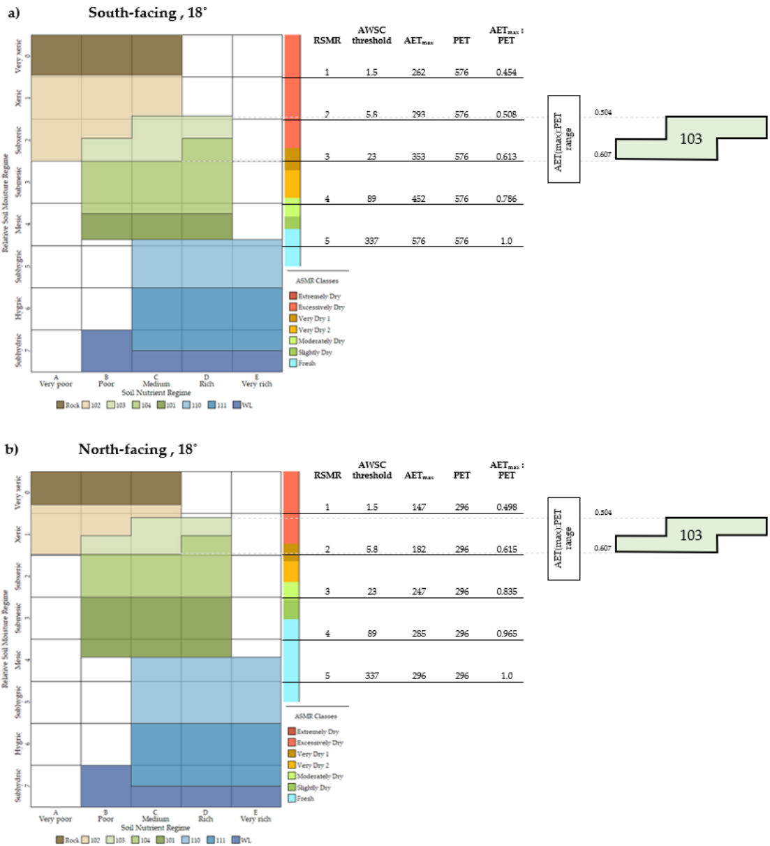
Figure 3-6. Edatopic grids for the ESSFdk1 variant (MacKillop et al., 2018) for south-facing and north-facing sites annotated with AWSC thresholds, AET max and PET values (in mm), and AET max :PET ratios at each upland RSMR class boundary. The range of AET max :PET ratios for the 103 site series is given at right in order to illustrate that it maintains the same AET max :PET ratio boundaries as the edatopic grid is shifted, which is also true for all other site series.
