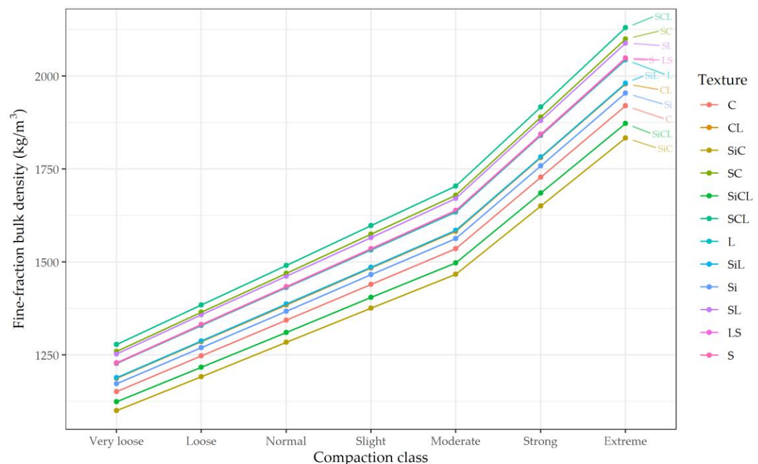
Figure 3-2. Translation of compaction class ratings to fine-fraction bulk density values by texture class.
