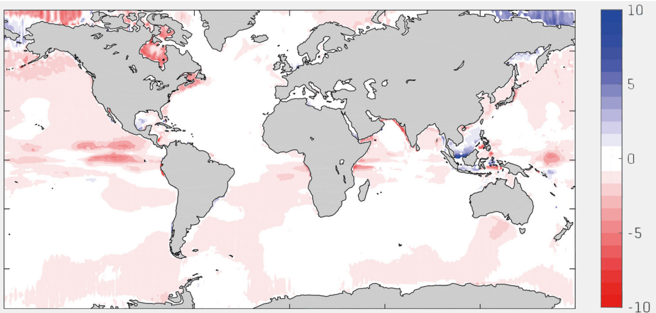
Percent change in dissolved ocean oxygen per decade since 1960. Schmidtke et al / GEOMAR
