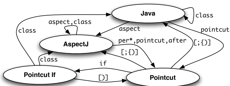
Figure 5.7 Lexical state transitions in the abc scanner
