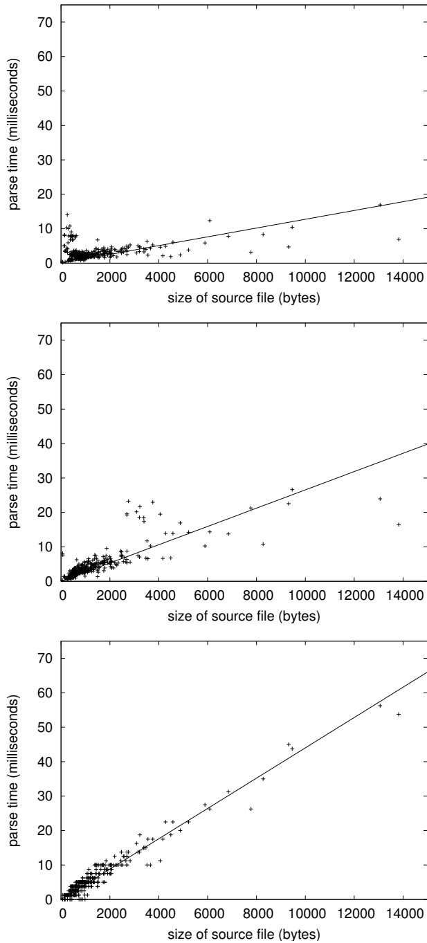
Figure 5.24 Benchmark of parsing AspectJ source files. Top to bottom: ajc, abc, sglr/ajc
