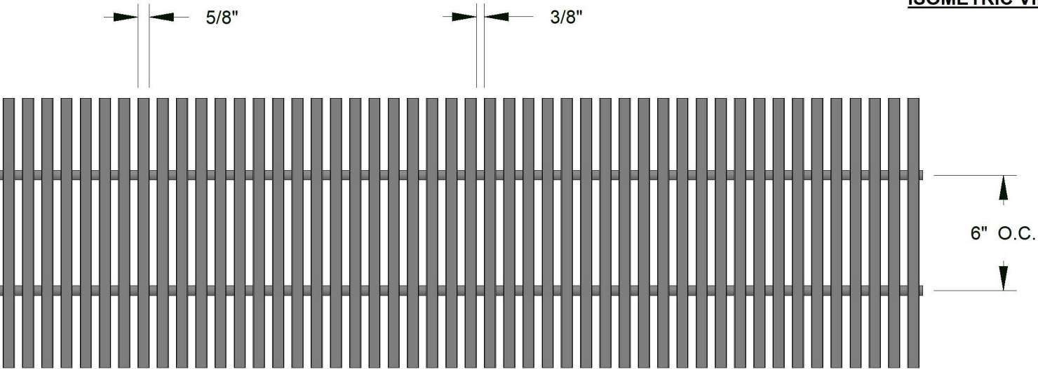
ISOMETRIC VIEW
