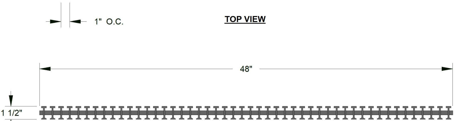
SIDE VIEW
