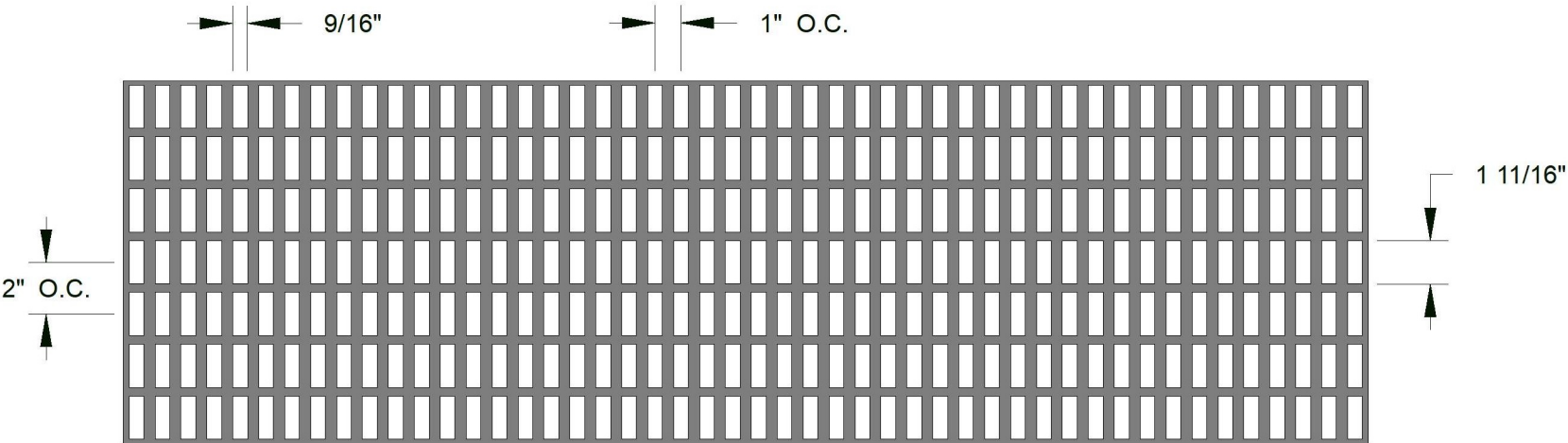
TOP VIEW
