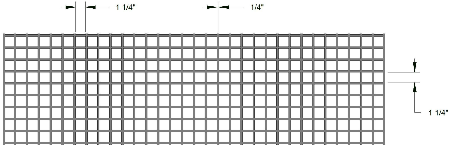
TOP VIEW
