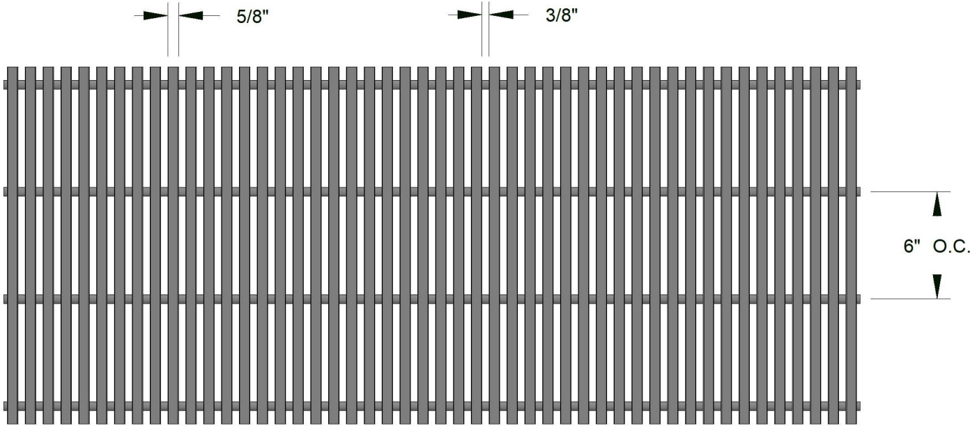
TOP VIEW
