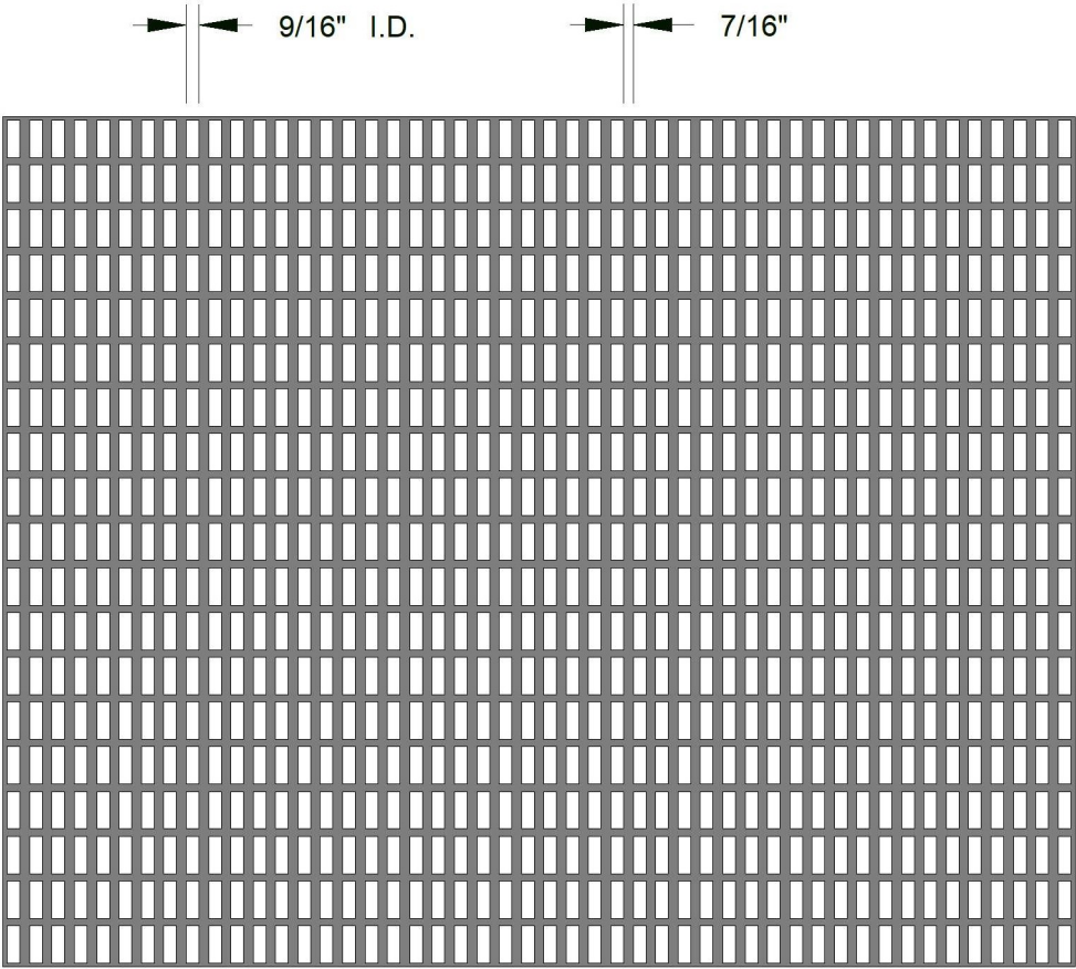
TOP VIEW
