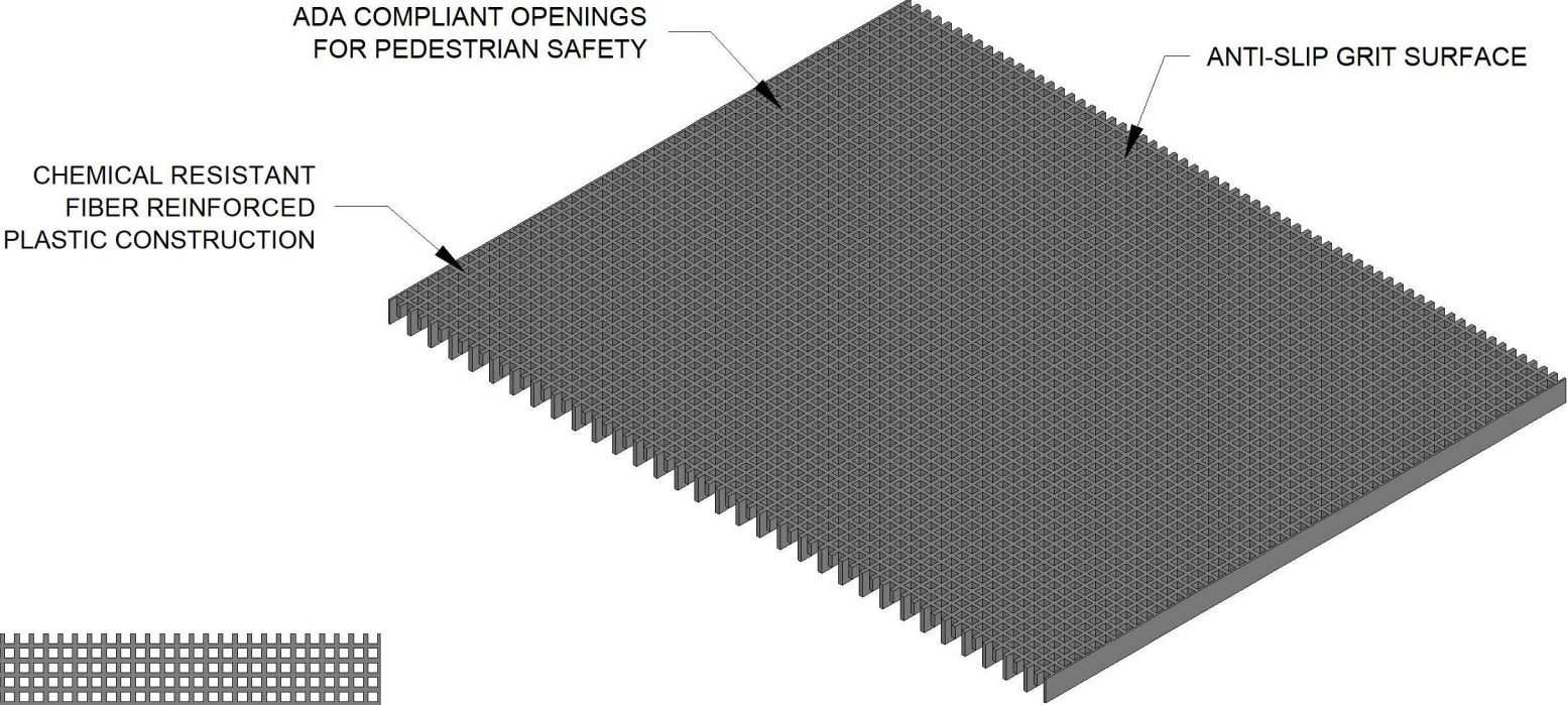
ISOMETRIC VIEW
