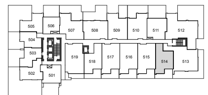
5TH FLOOR
