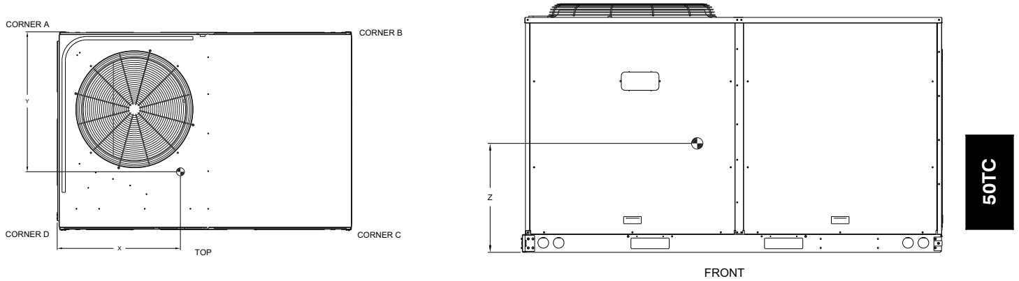
Fig. 10 - Dimensions 50TC-14
