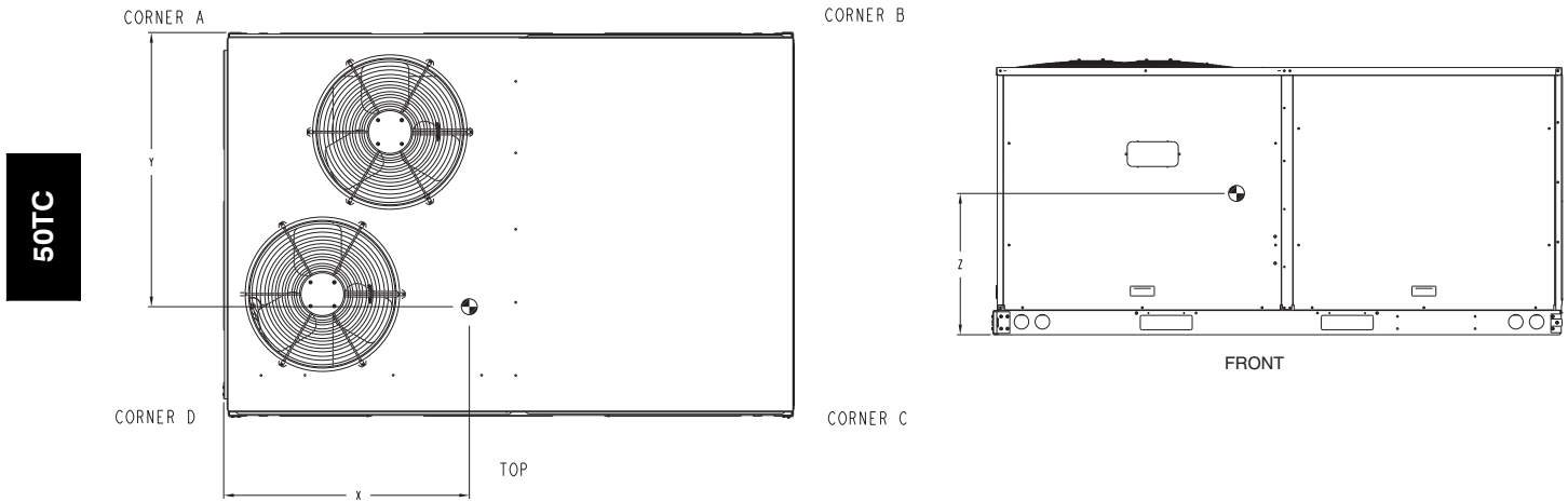
Fig. 6 - Dimensions 50TC 08-12
