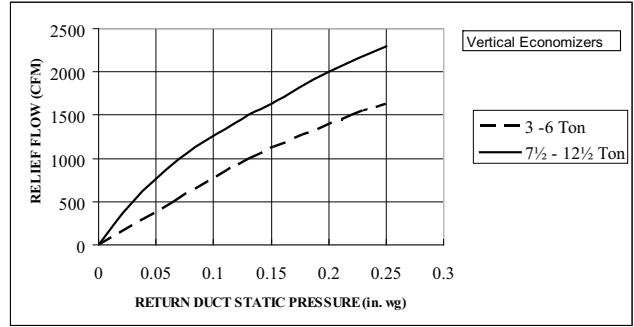
Fig. 16 - Barometric Relief Flow Capacity
