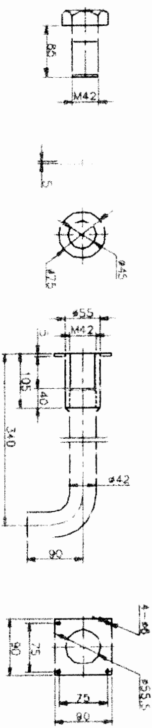
M42 Tender Anchor Bolt Set
