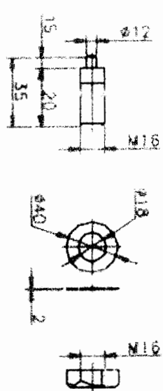
M16 Rod Fixing Bolt Set
