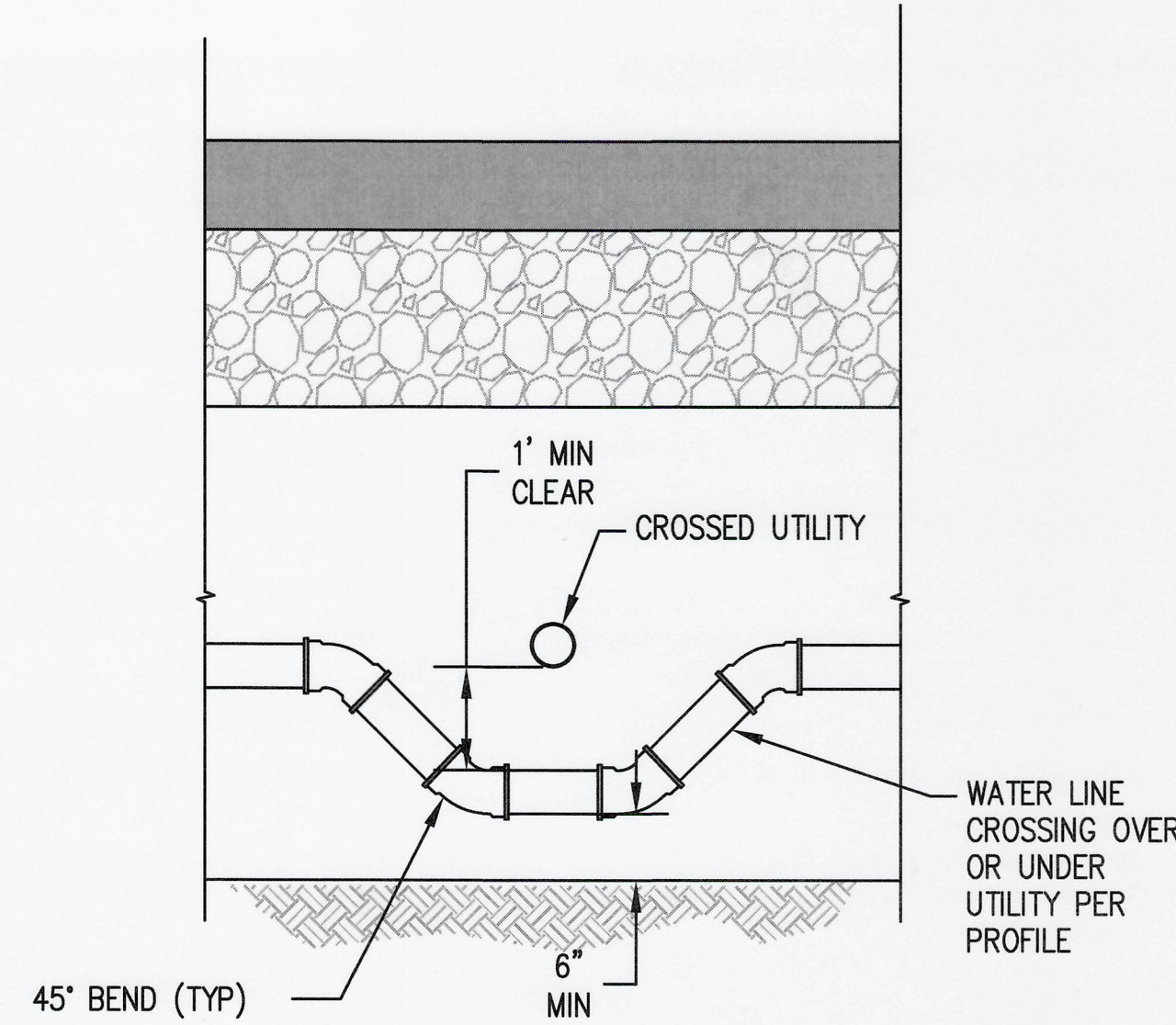
2 UTILITY CROSSING C1.7 NTS
