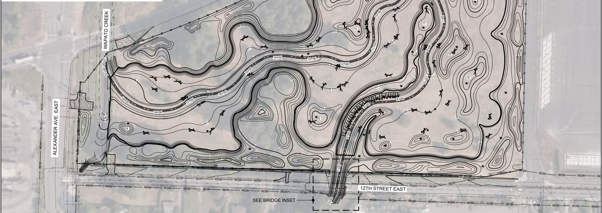
FIGURE 8. GRADING PLAN
