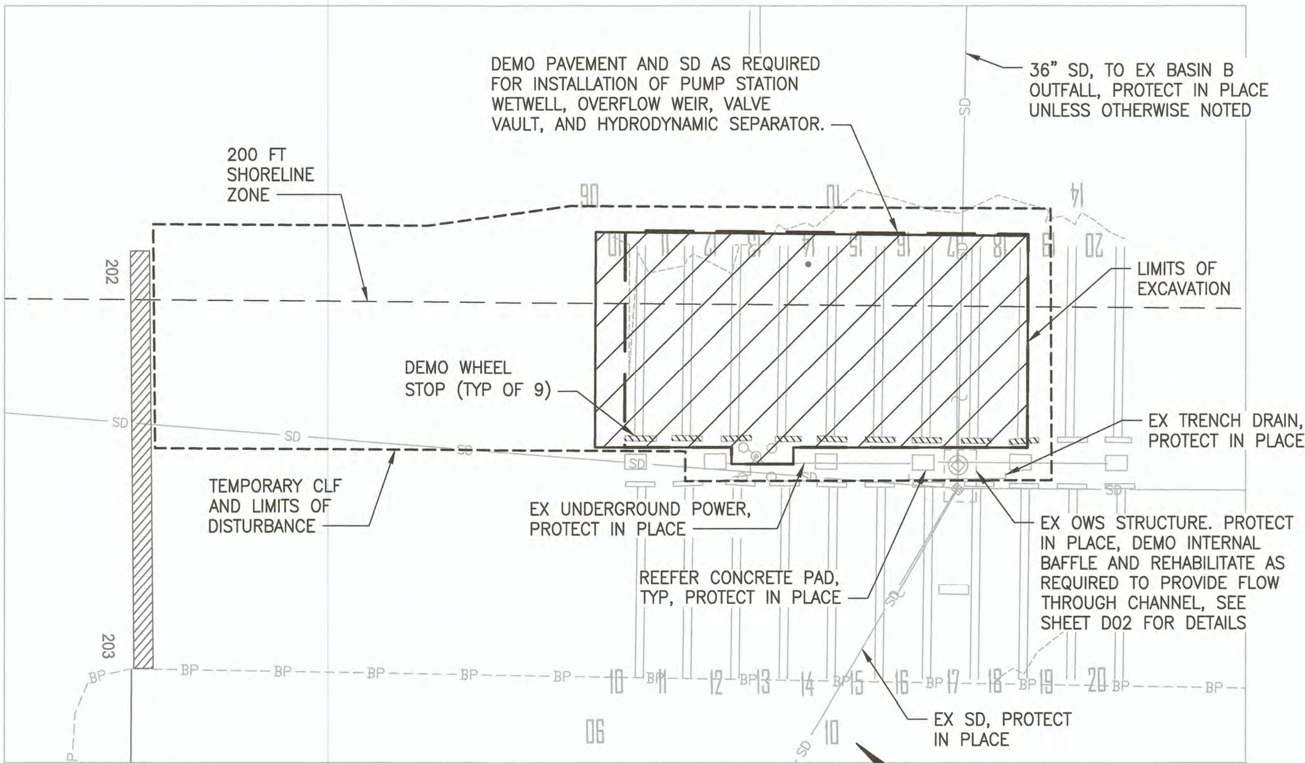
BASIN B - DEMO PLAN
