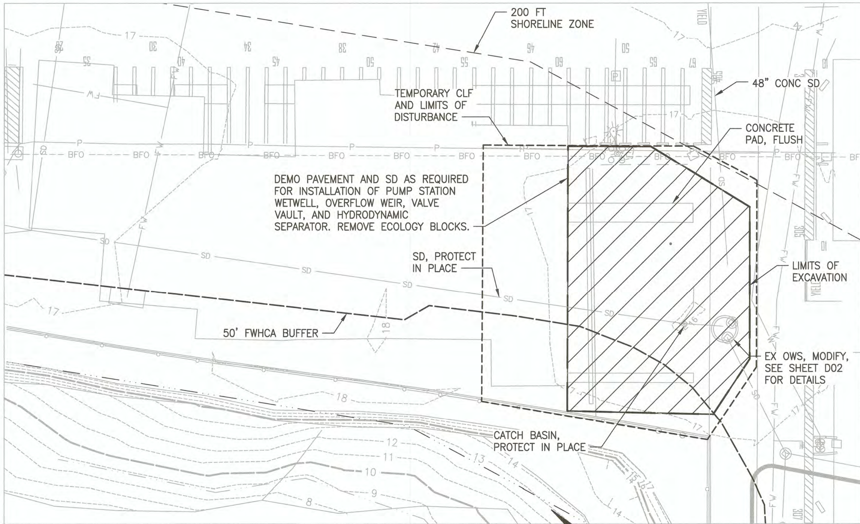
BASIN C - DEMO PLAN
