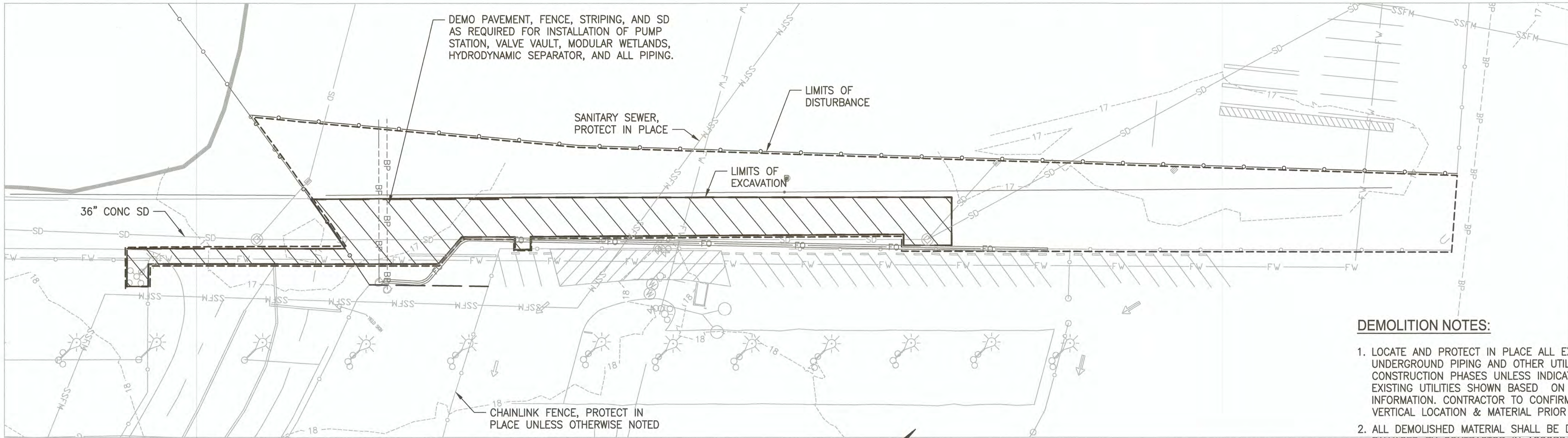
BASIN A - DEMO PLAN
