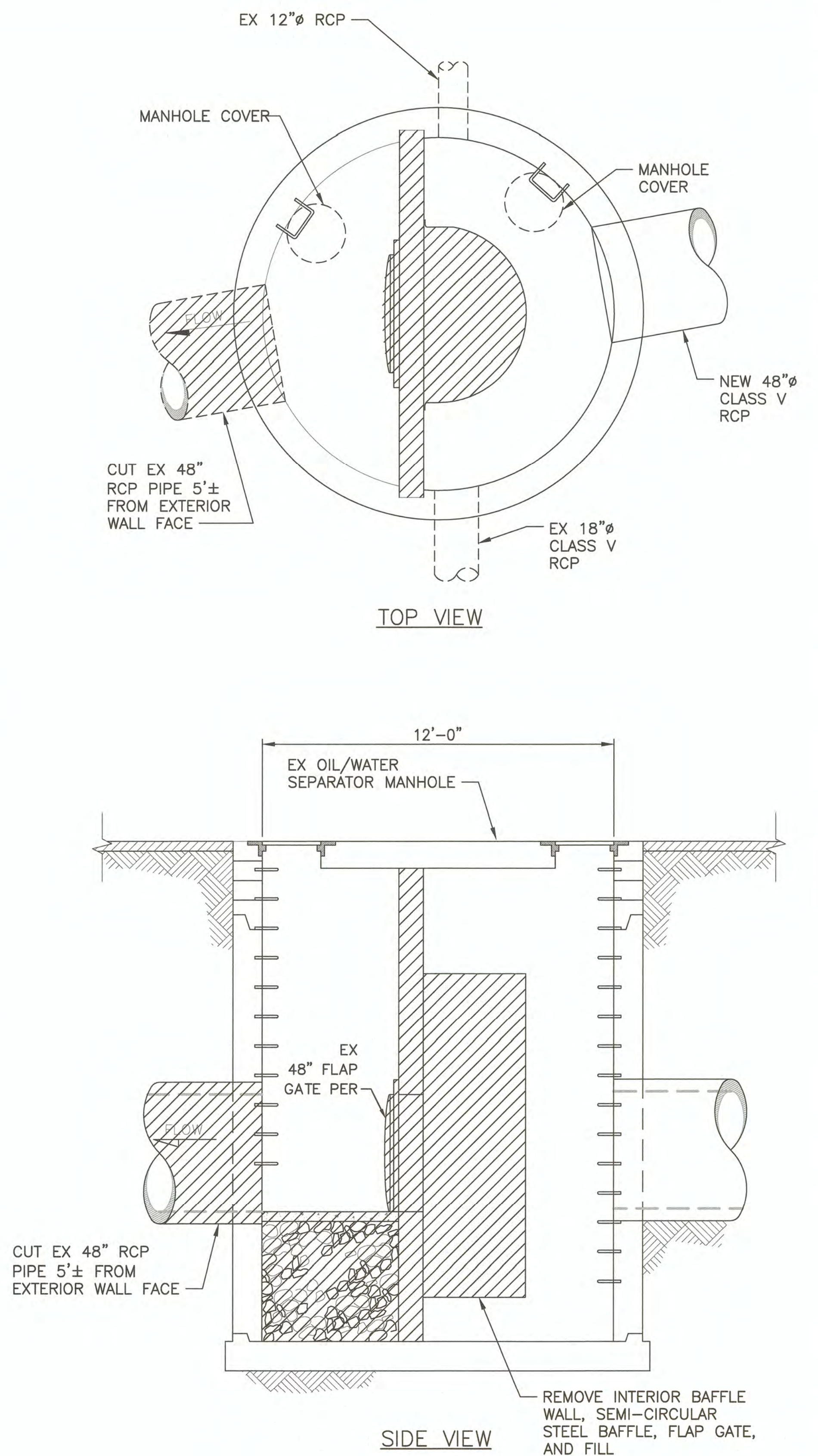
2 M03 EXISTING BASIN C OIL/WATER SEPARATOR DETAIL SCALE: NOT TO SCALE
