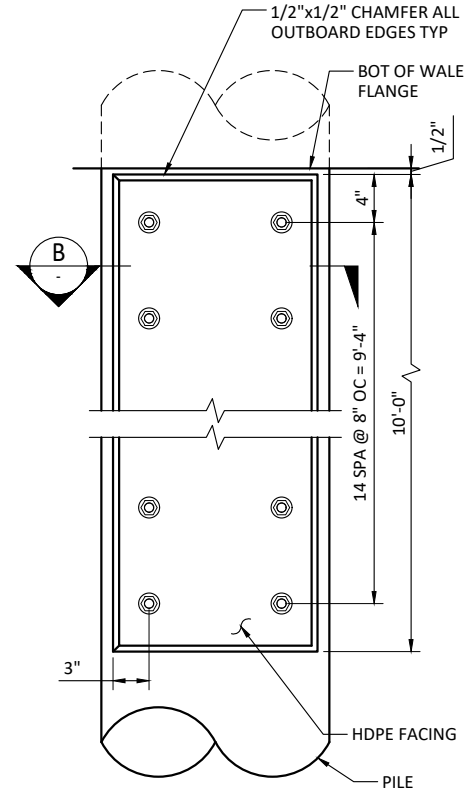
A SECTION - PILE FACING SCALE: 3/4" = 1'-0"
