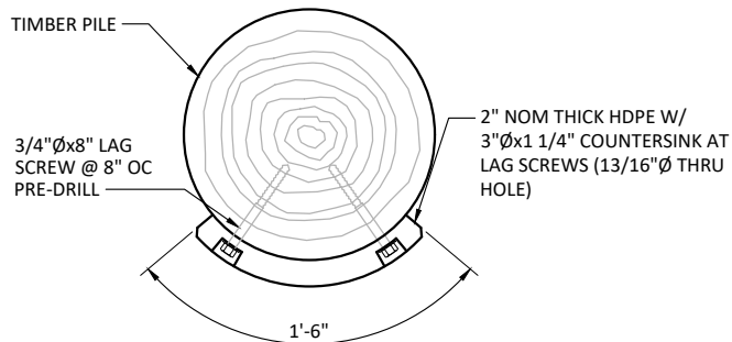
B SECTION - PILE FACING SCALE: 3/4" = 1'-0"
