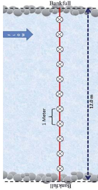
Figure 30. Example of a cross-section layout. In this example, distance between samples is 1 m, because the bankfull width is 12 m. Particle sample location is shown with a circle and crosshairs.
