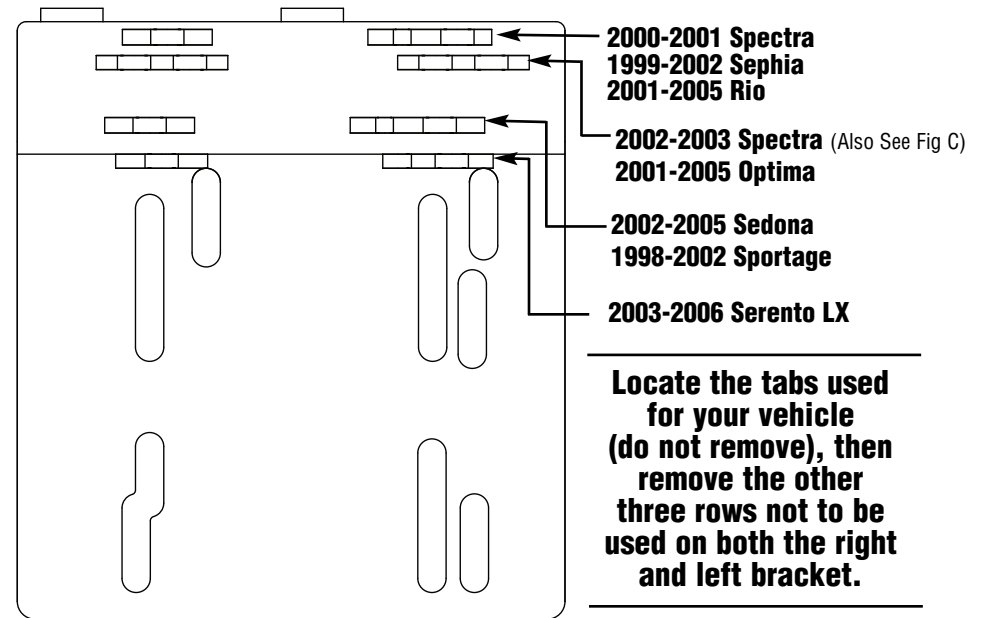
VIEW OF RIGHT SIDE BKT.
