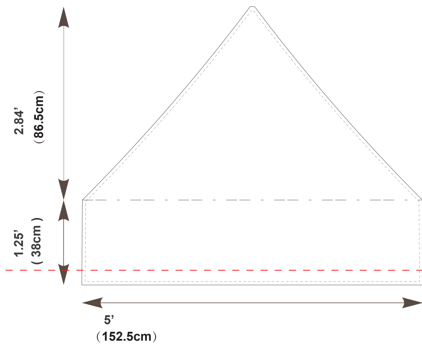
RIGHT VALANCE PANEL
