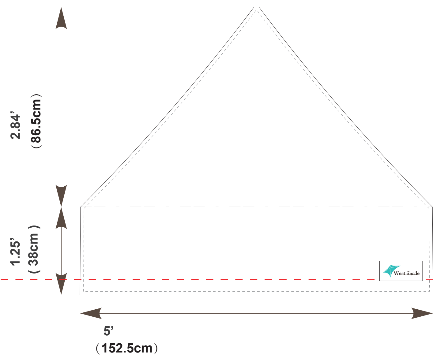
BACK VALANCE PANEL
