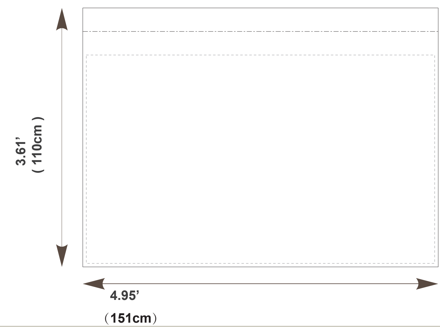
LEFT HALF-WALL OUTSIDE PANEL
