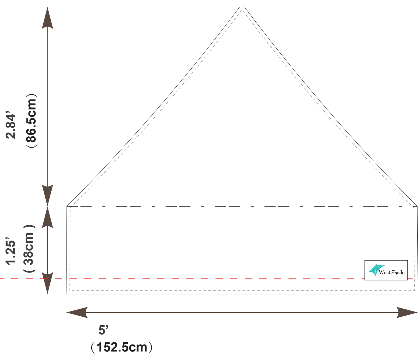
FRONT VALANCE PANEL
