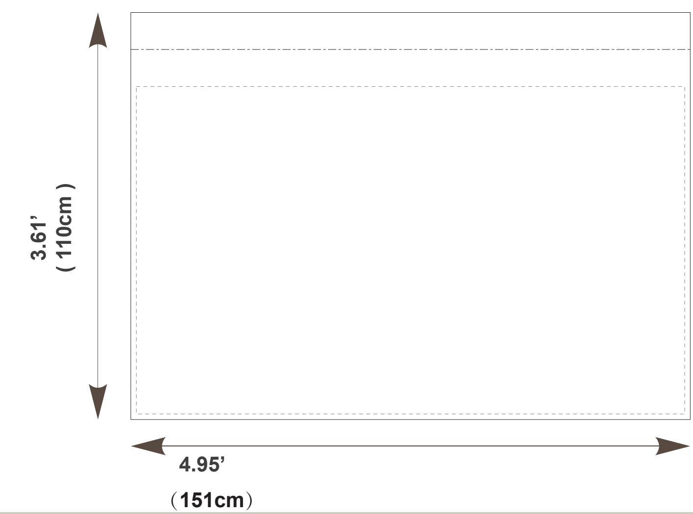
BACK HALF-WALL OUTSIDE PANEL
