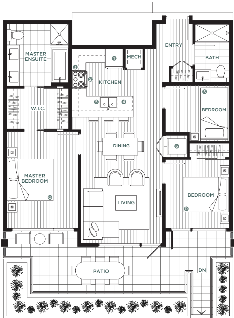
VARIANCE PLAN - BLDG1 #103
