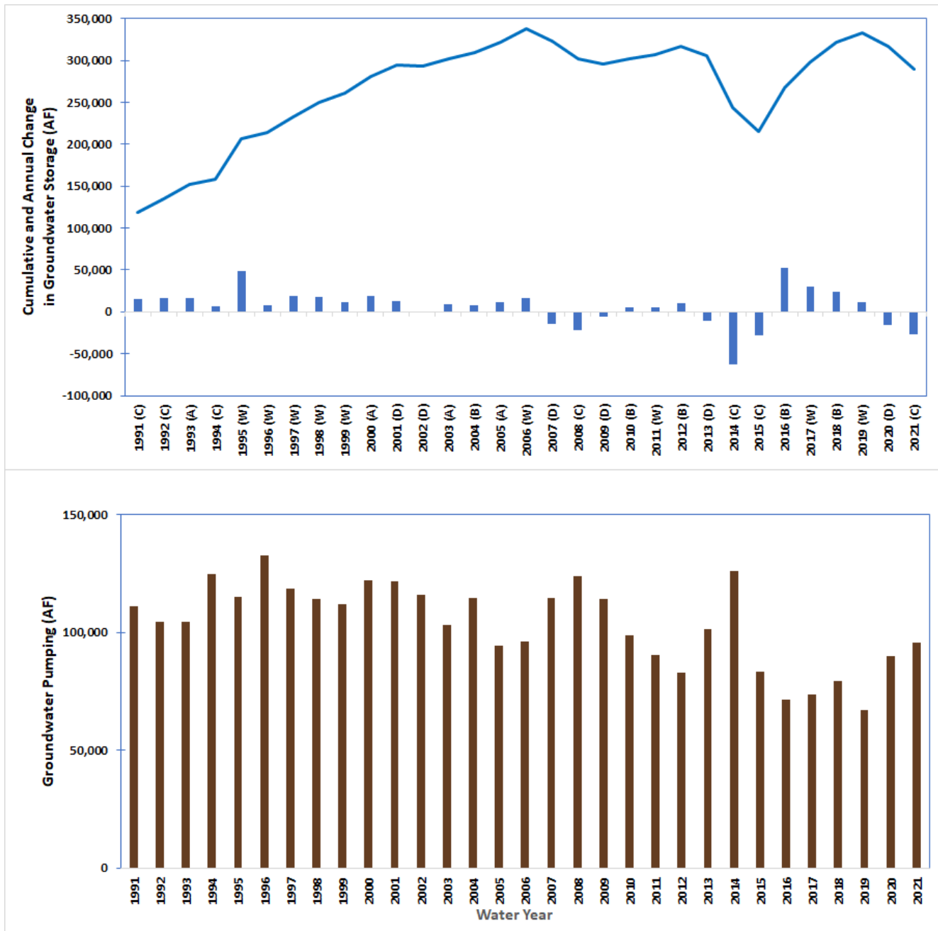
Figure 9. Groundwater Use and Change in Storage in the Santa Clara Subbasin
