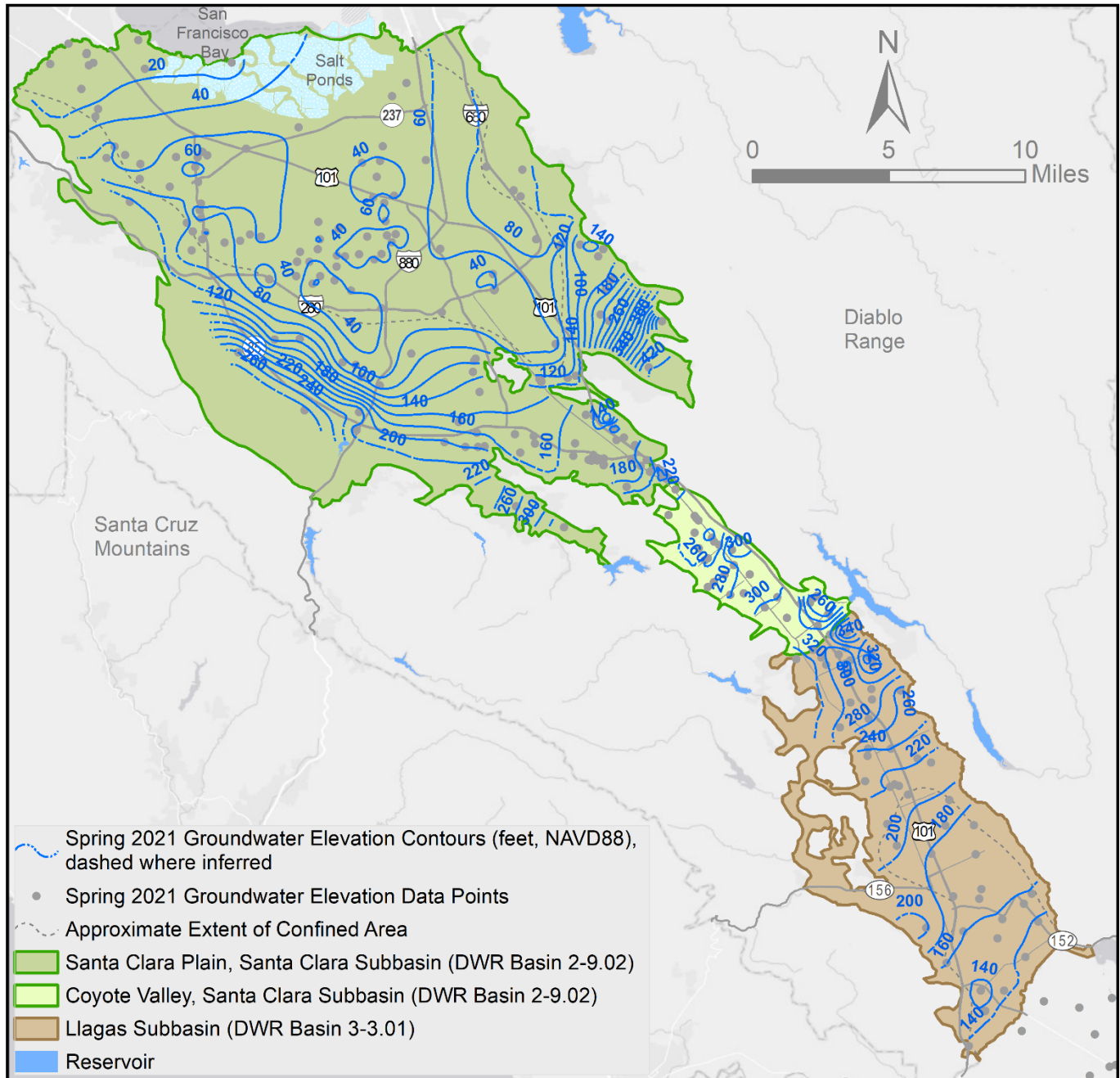
Figure 2. Spring 2021 Groundwater Elevation Contours
