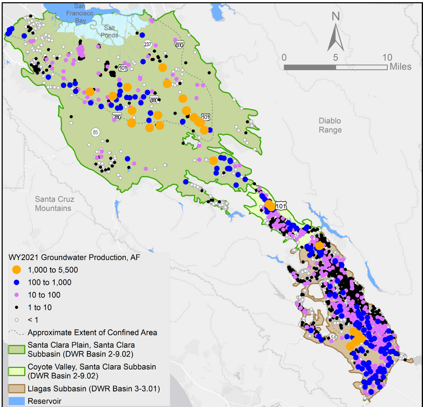
Figure 7. WY 2021 Groundwater Pumping in the Santa Clara and Llagas Subbasins
