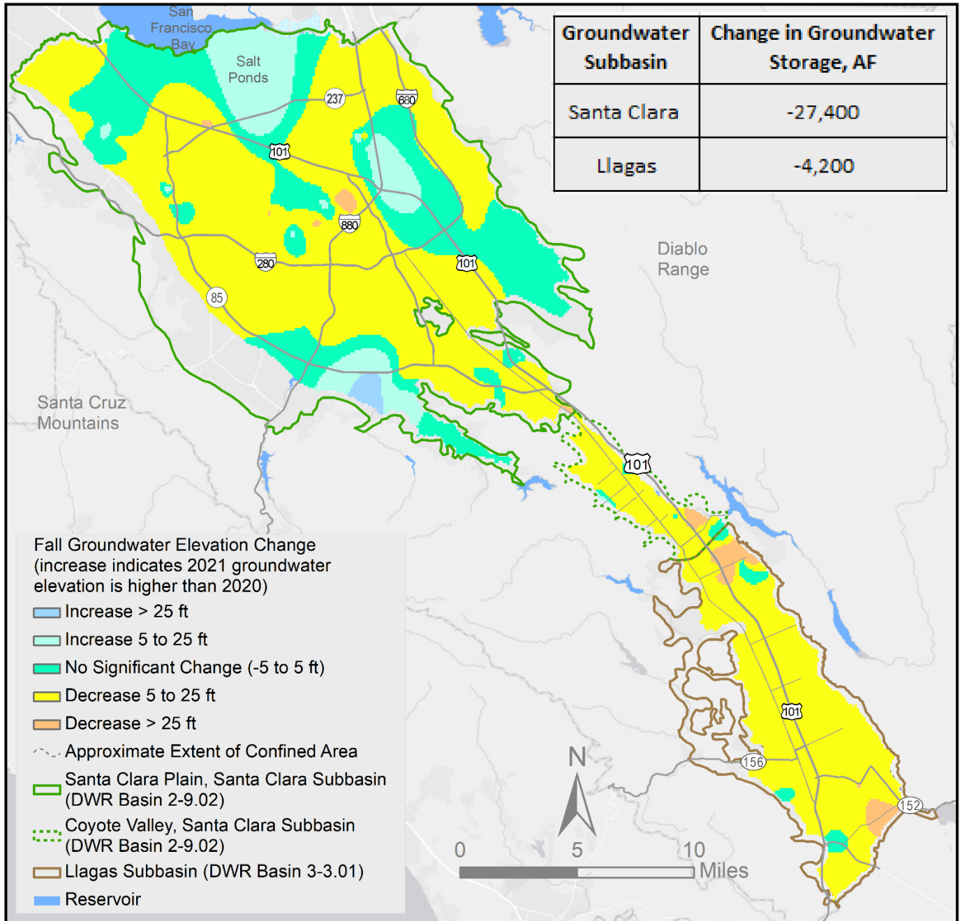
Figure 8. Change in Groundwater Elevation and Storage from October 2020 to September 2021
