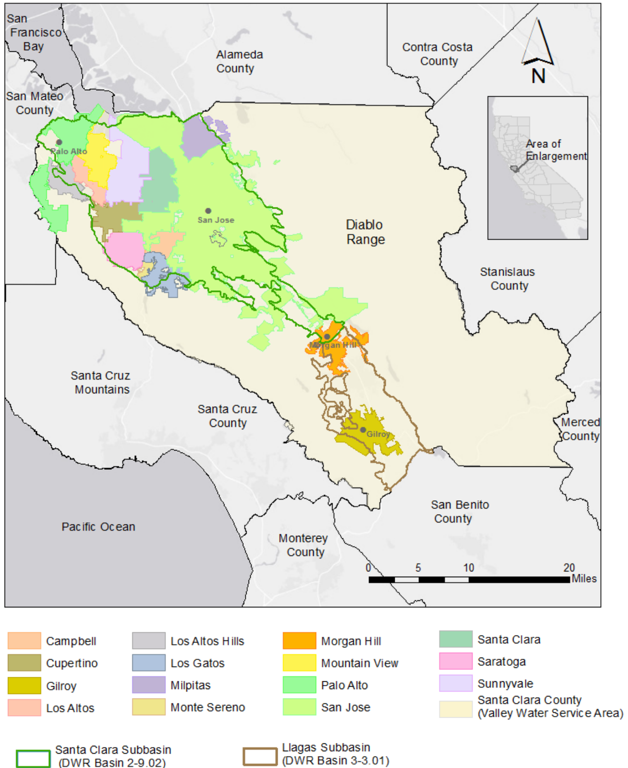
Figure 1. Santa Clara and Llagas Subbasin Location Map
