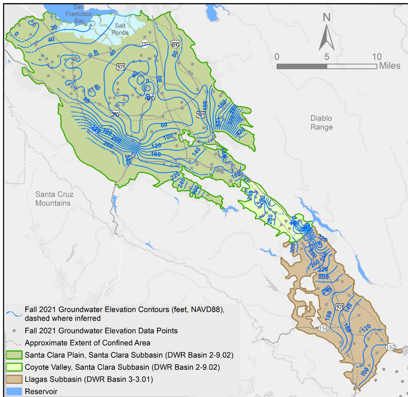
Figure 3. Fall 2021 Groundwater Elevation Contours
