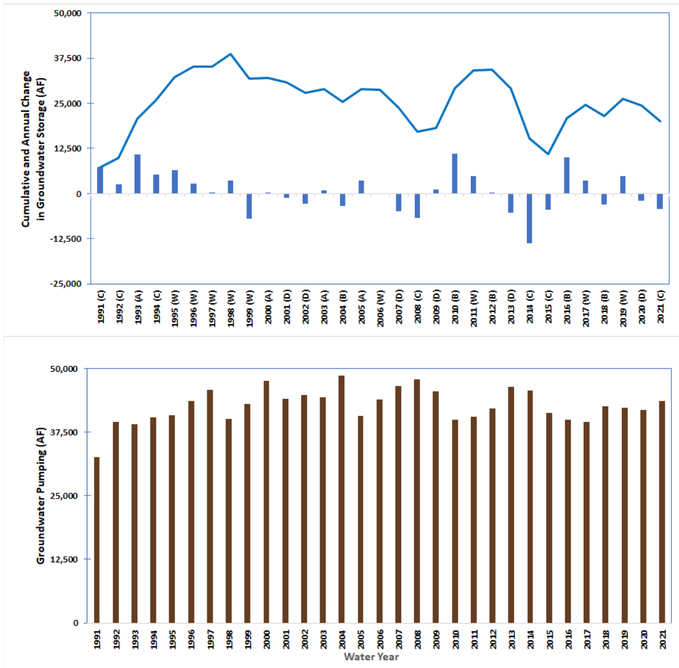
Figure 10. Groundwater Use and Change in Storage in the Llagas Subbasin
