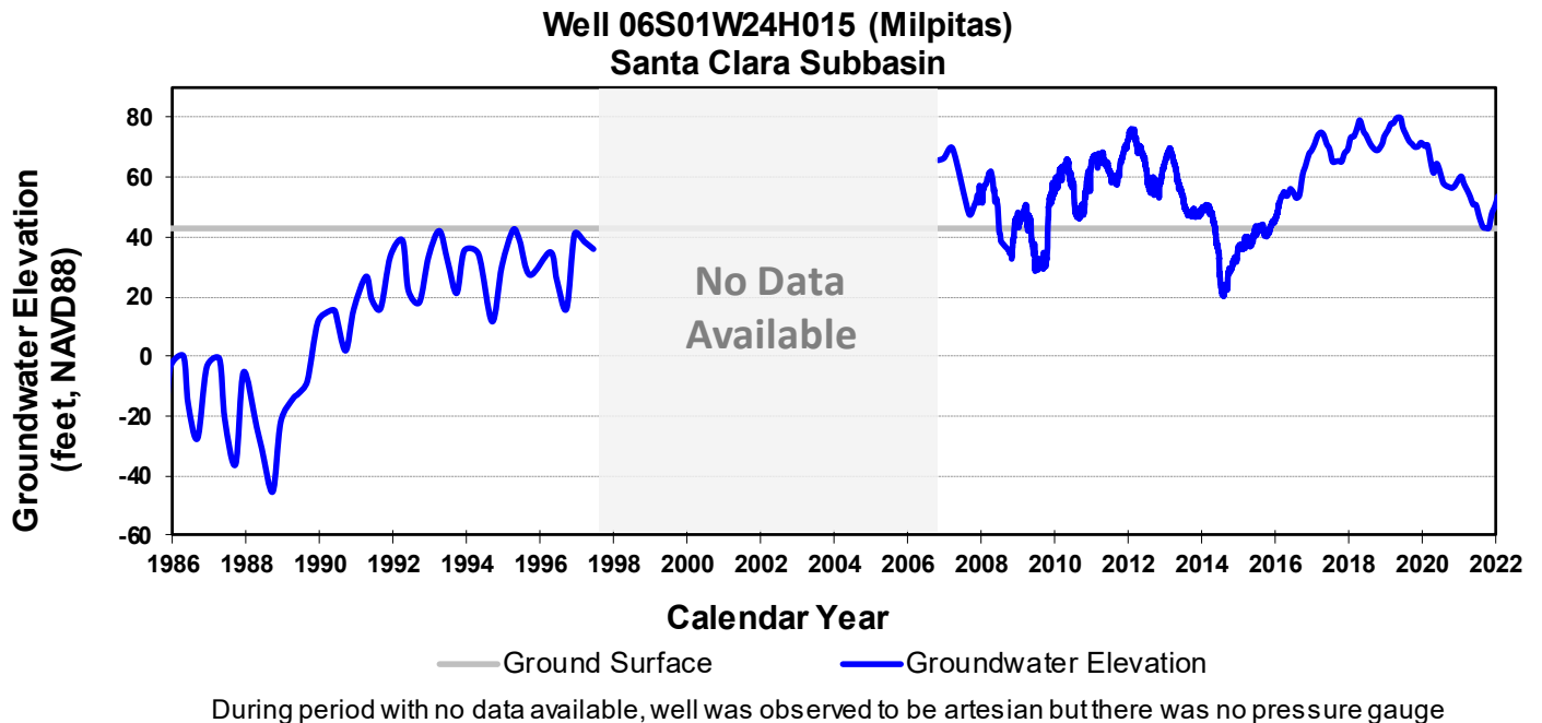
Figure 5. Hydrographs at Regional Groundwater Elevation Monitoring Wells
