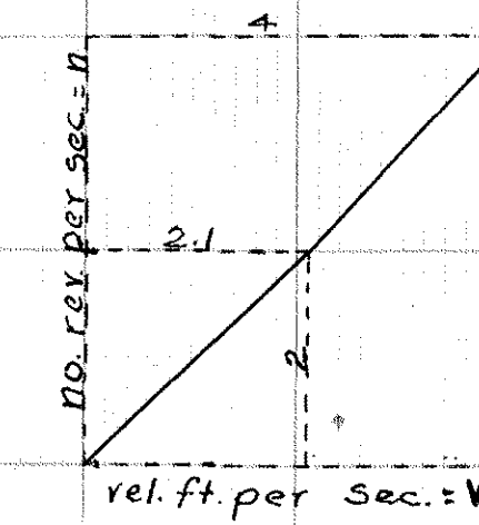
RATING CURVE FOR K & E CURRENT METER #362
